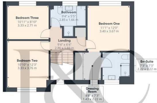
Floor 1 Building 1
